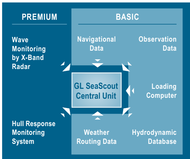
For an optimal routing GL SeaScout Central Unit requires information from different systems onboard
